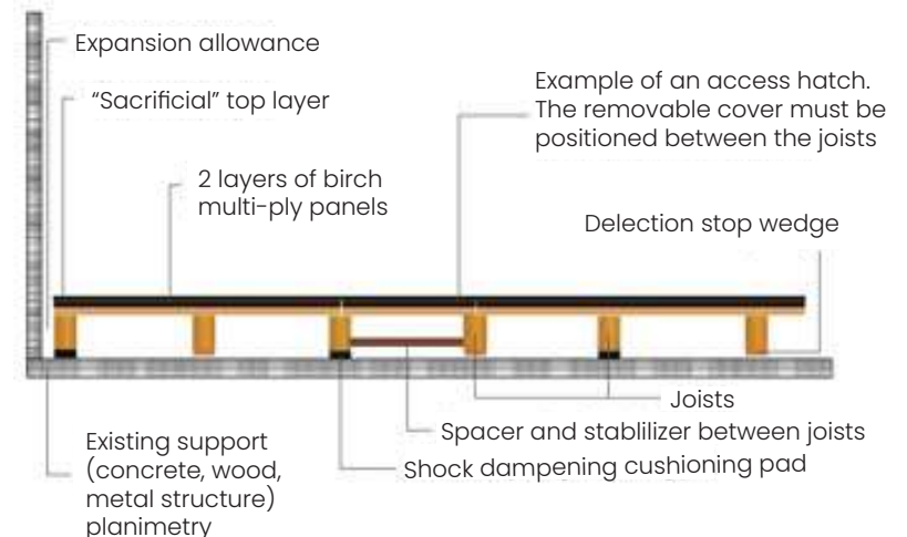
Cross section of Harlequin Stage System
